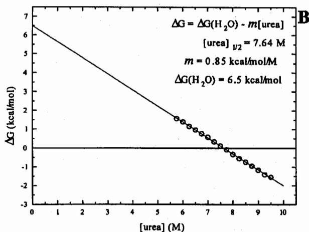
Fig. 2. A: Urea denaturation curve for RNase Sa determined at 25°C, pH 5.0, 30 mM sodium acetate buffer as described by Pace et al. 50 The solid line is based on an analysis of the data by using Eq. (4). B: \Delta G (o) as a function of urea molarity. The \Delta G values were calculated from the data in the transition region as described in the text. The \Delta G(\text{H}_2\text{O}) and m values can be determined by fitting the data in part B to Eq. (3), or by analyzing the data in part A with Eq. (4).
